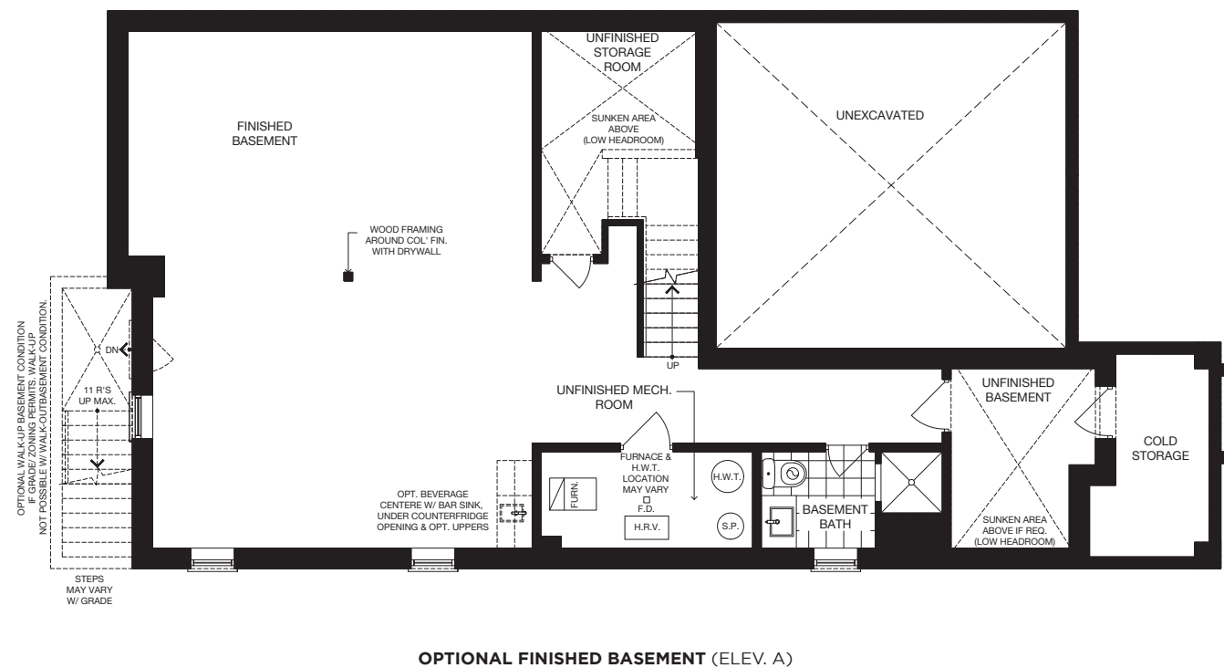
OPTIONAL FINISHED BASEMENT (ELEV. A)
