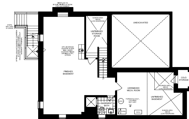
OPT. FINISHED BASEMENT A
