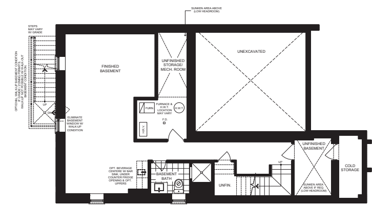
OPT. FINISHED BASEMENT A
