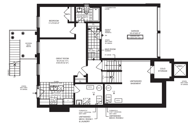
LOWER FLOOR PLAN W/ ACCESSORY UNIT A
