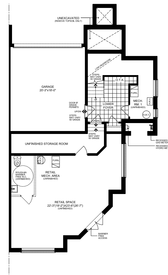
LOWER LEVEL C1
