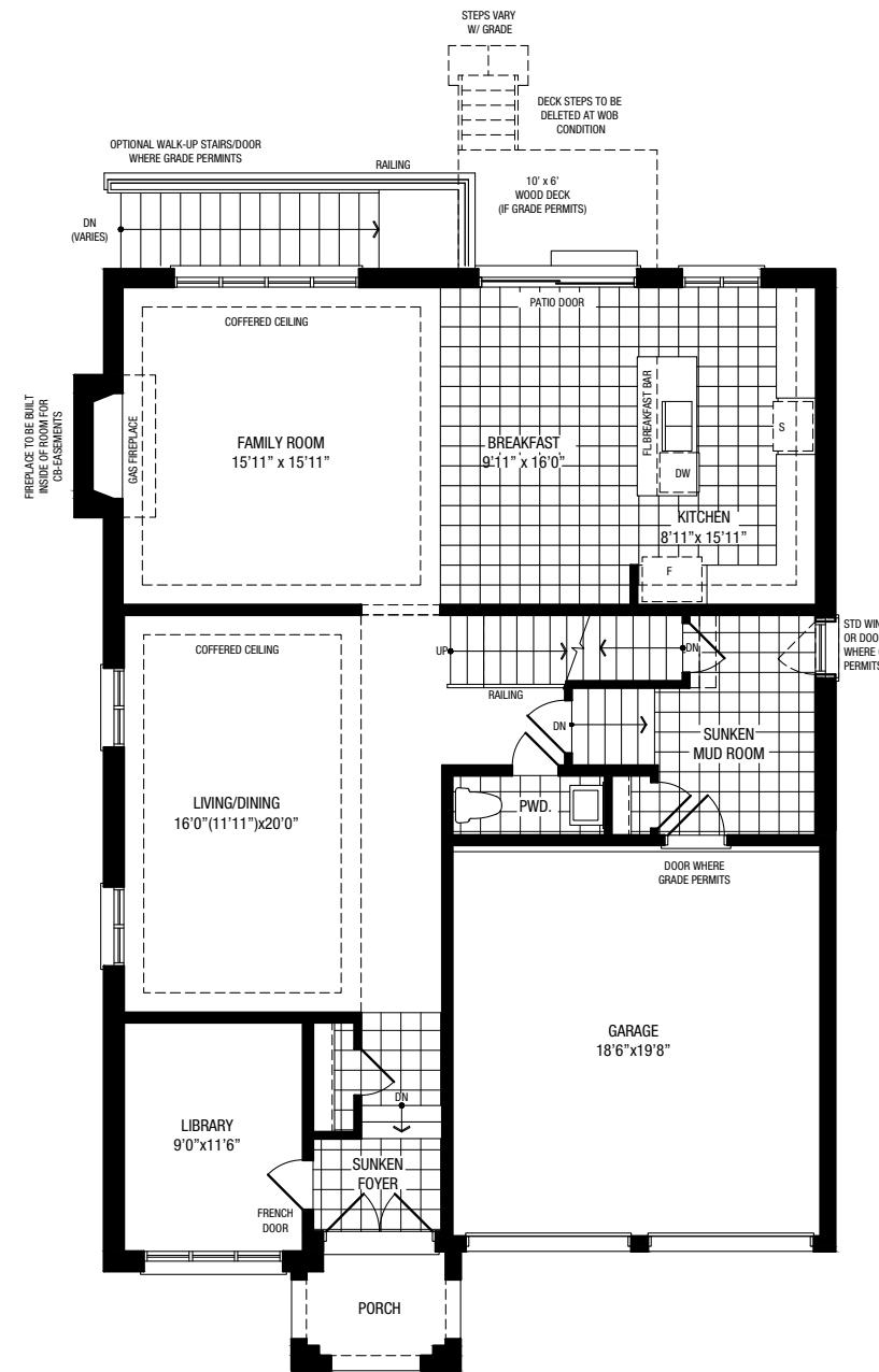
GROUND FLOOR ELEV. C
