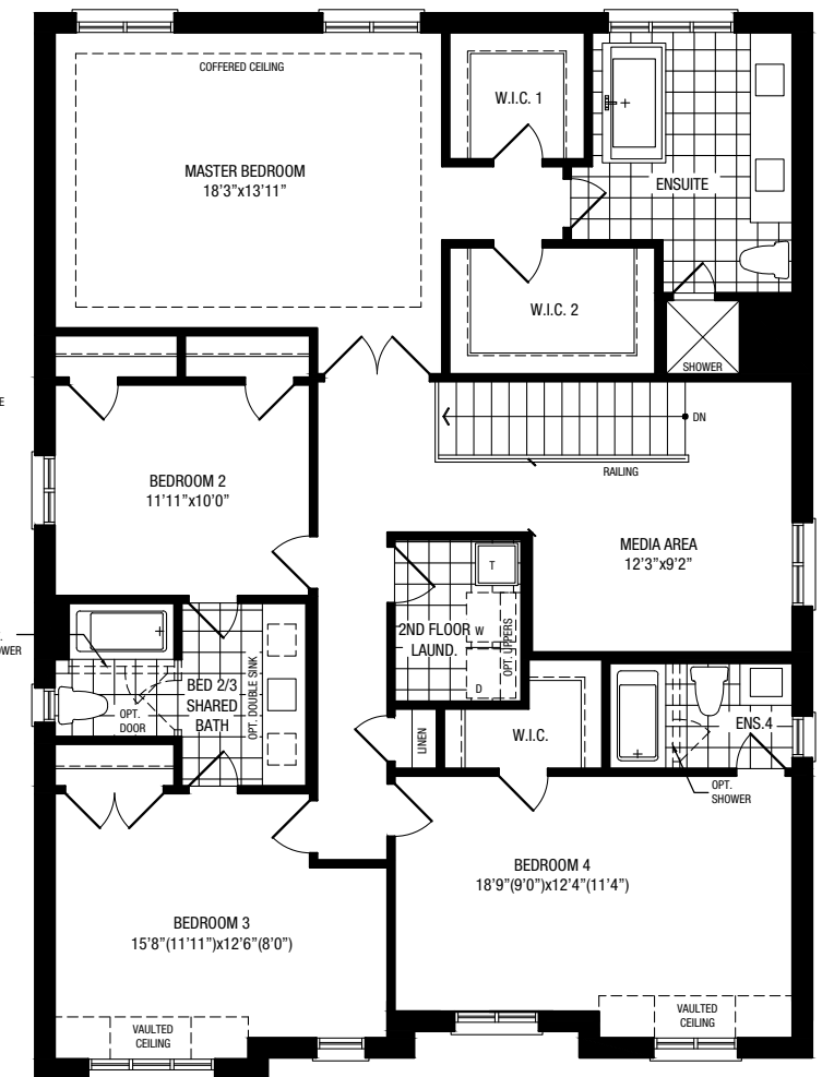
SECOND FLOOR ELEV. C
