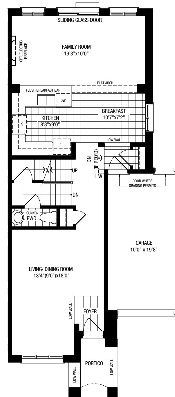
GROUND FLOOR ELEV. B
